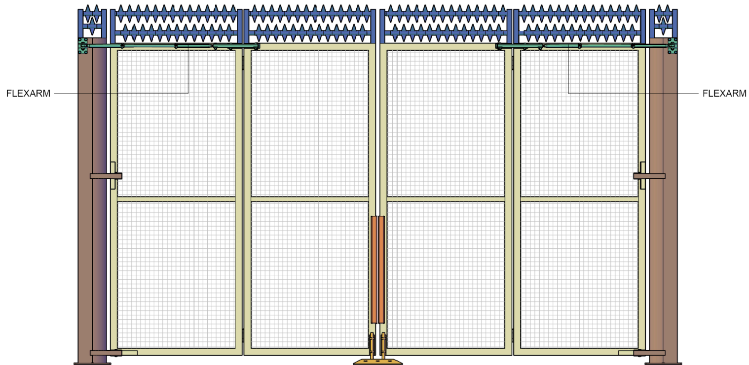
TYPICAL QUICKFOLD VEHICLE GATE SYSTEM ELEVATION VIEW FROM INSIDE PROPERTY SCALE: 1/2" : 1'
