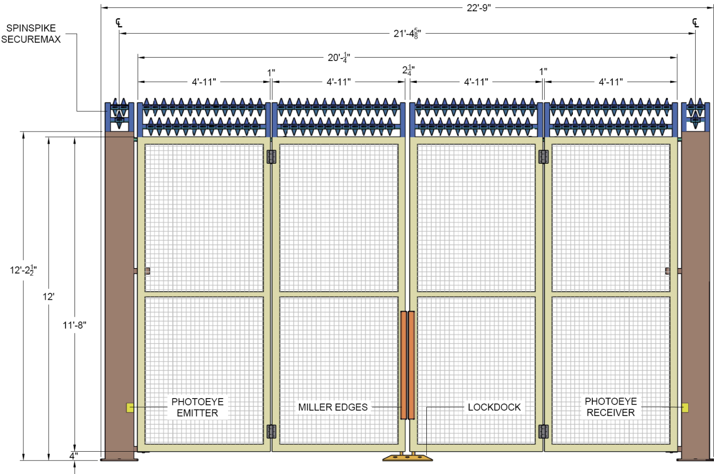
TYPICAL QUICKFOLD VEHICLE GATE SYSTEM ELEVATION VIEW FROM OUTSIDE PROPERTY SCALE: 1/2" = 1'
