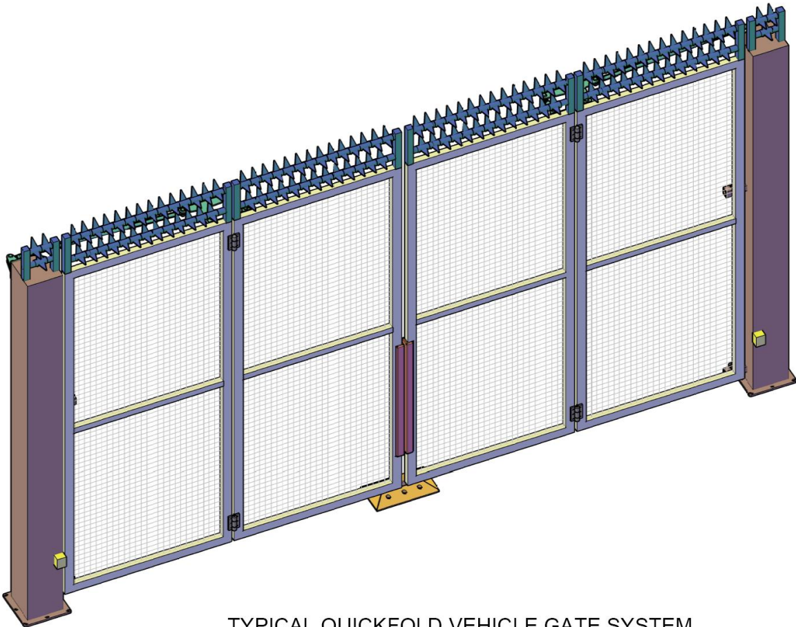
TYPICAL QUICKFOLD VEHICLE GATE SYSTEM PERSPECTIVE VIEW FROM OUTSIDE PROPERTY SCALE: 1/2" : 1'
