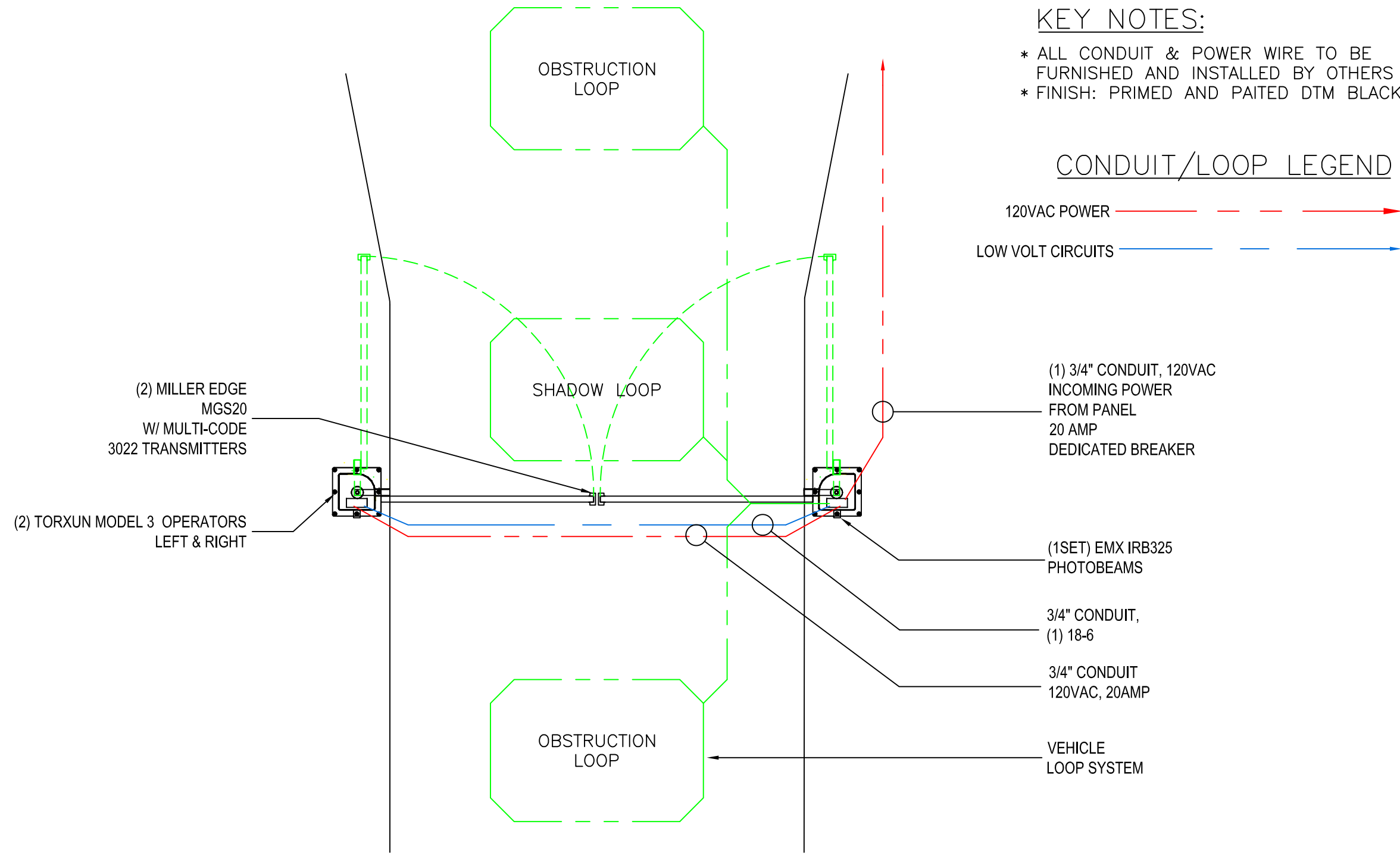
PLAN VIEW: BI-PARTING SWING GATES SCALE: 3/8" = 1' OUTSIDE LOOKING IN
